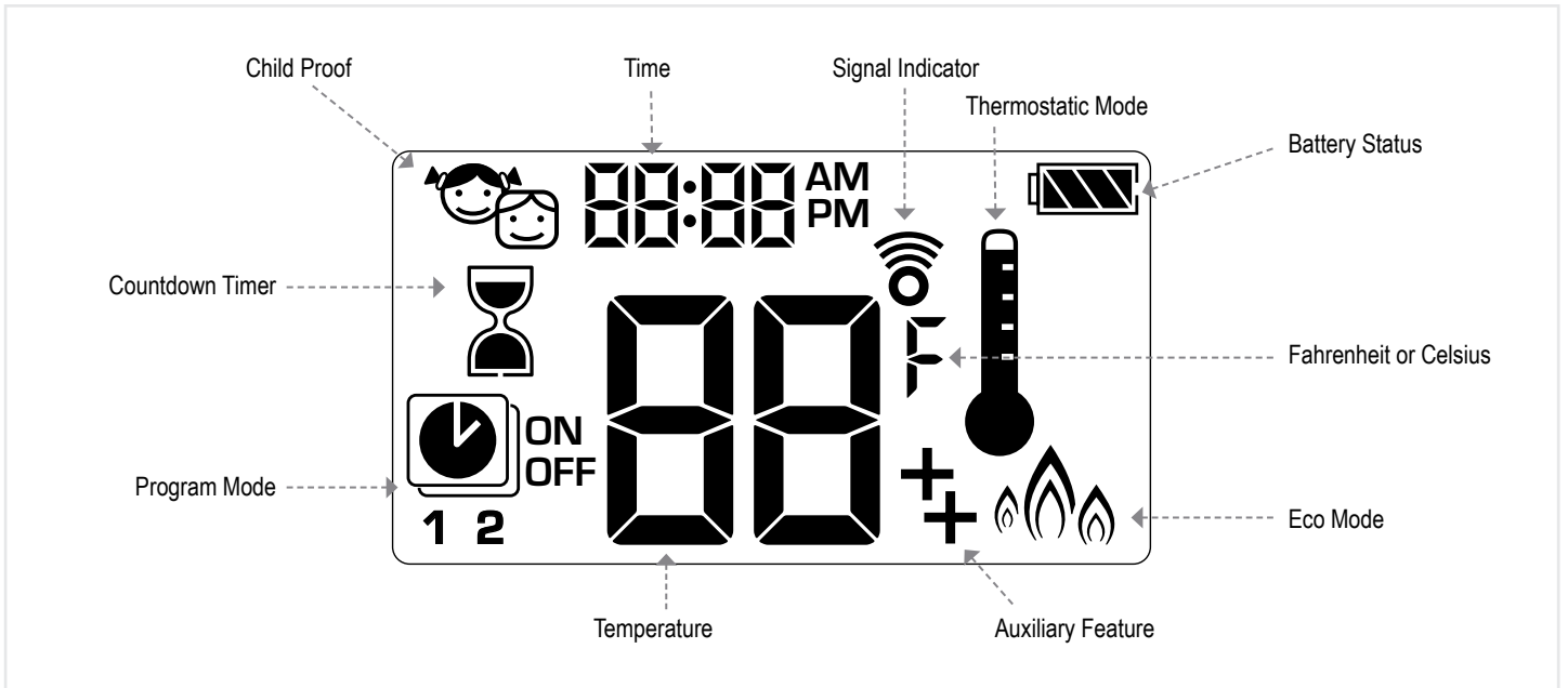
Figure 21: 8-symbol Display
