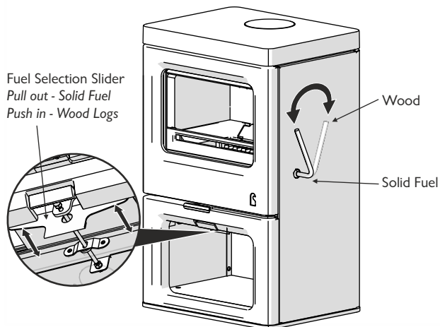
Fig.1 Operating the multi grate
