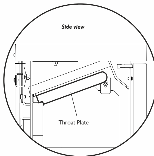
Fig.6 Throat Plate Location
