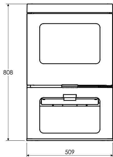
Standard Model
