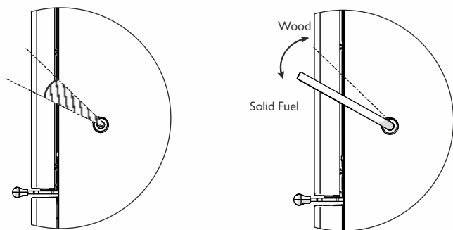
Fig.2 Riddling tool
