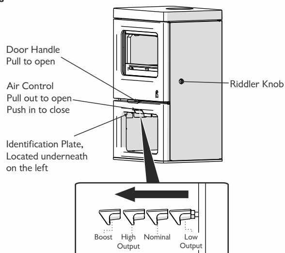
Fig. 3 Stove controls
