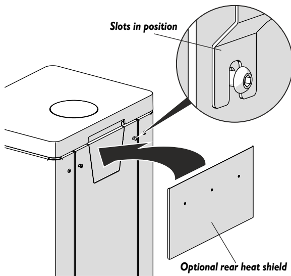
Fig. 12. Fitting the optional rear heat shield.
